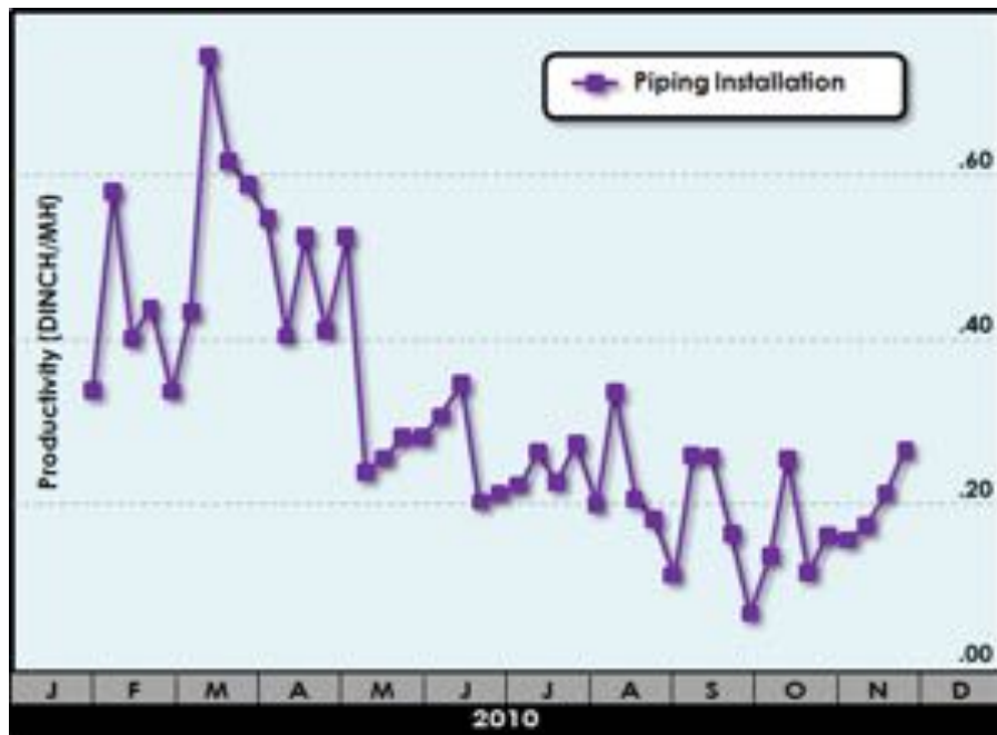
Figure 3. Piping Installation Labor Productivity Rate
